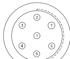
SOLDER CUP SIDE J1
